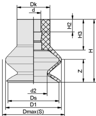
Design data FGA 11 SI-MD-55 N016
