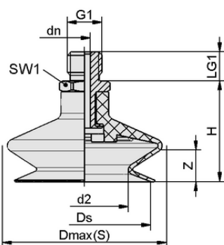
Design data FSGA 4 SI-CO-55 M3-AG
