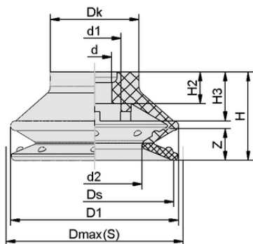
Design data SDC1 30 PU 30/60 N043
