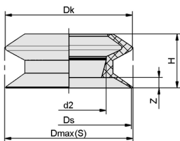
Design data FLSA 40 SI-HD-65
