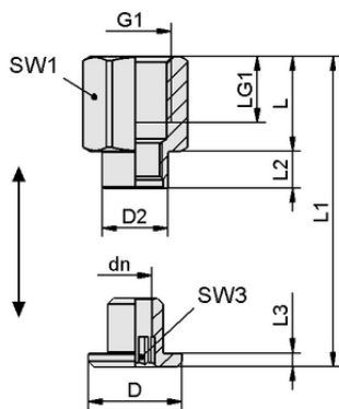
Design data SC 050-AR G1/4-IG MOD
