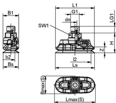
Design data SPOB1f 60x25 SI-55 G1/4-AG
