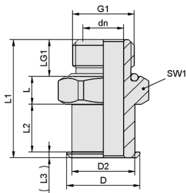
Design data SC 090 NPT1/4-AG
