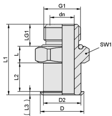
Design data SC 080 NPT3/8-AG
