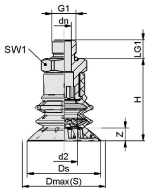
Design data SPB2f 40 SI-55 G1/4-AG
