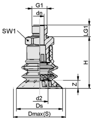
Design data SPB2f 40 SI-55 G1/8-AG
