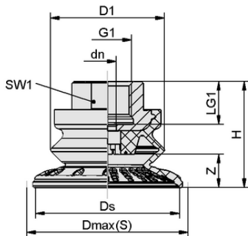
Design data SAB 80 HT1-60 G1/2-IG
