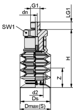
Design data SPB4 40 SI-55 G1/2-AG
