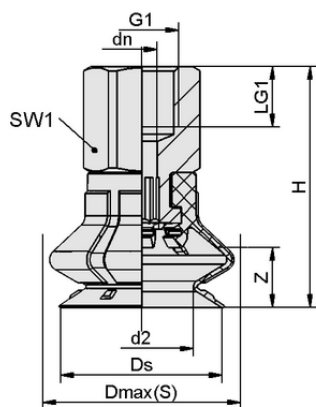
Design data SPB1 25 ED-65 G1/8-IG
