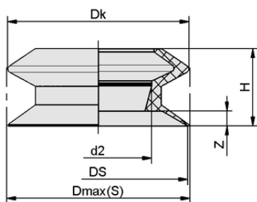
Design data FLSA 50 SI-HD-65
