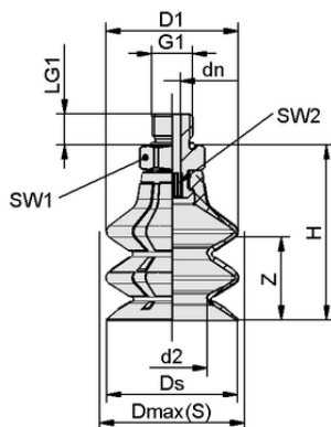
Design data SPB2 50 ED-65 G1/4-AG
