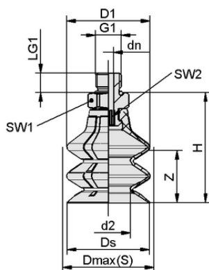
Design data SPB2 20 ED-65 G1/8-AG
