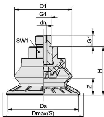
Design data SAB 50 HT2-65 G1/4-AG
