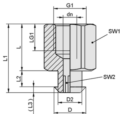
Design data SC 030 M5-IG
