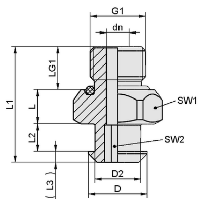
Design data SC 040 G1/4-AG
