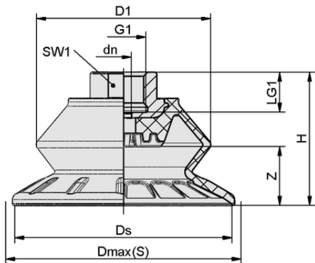
Design data SAB 80 HT2-65 G3/8-IG
