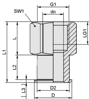
Design data SC 080 G1/4-IG
