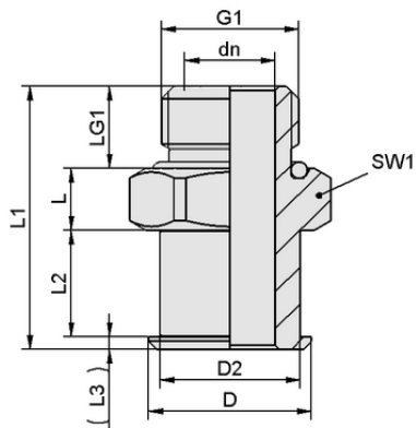
Design data SC 080 G1/4-AG
