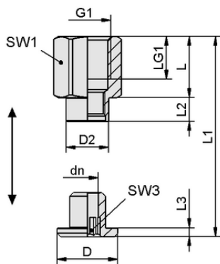
Design data SC 065 G1/4-IG L MOD
