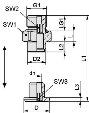
Design data SC 065 G1/4-AG L MOD
