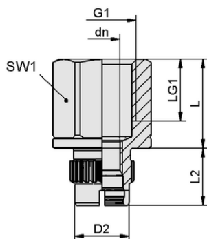
Design data SC-A 055-AR NPT3/8-IG L
