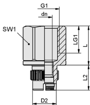
Design data SC-A 055-AR G1/4-IG L
