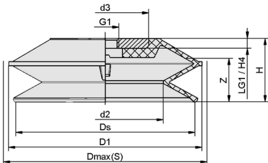
Design data FSGPL 150 HT1-60 G1/2-IG
