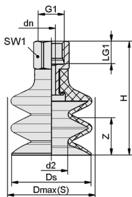
Design data FSG 4 NBR-CO-55 M5-IG
