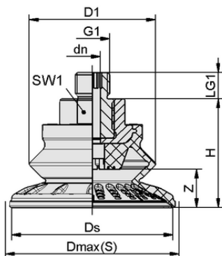
Design data SAB 125 HT1-60 G1/4-AG
