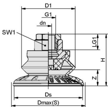
Design data SAB 30 HT1-60 G3/8-IG
