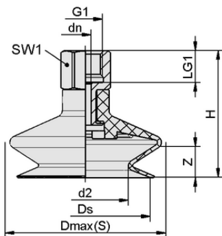
Design data FSGA 6 HT1-60 M5-IG
