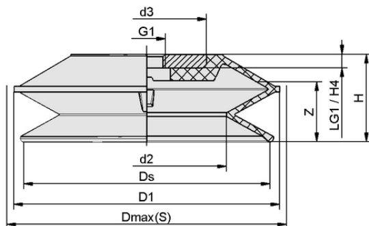
Design data FSGPL 100 NBR-55 G1/2-IG
