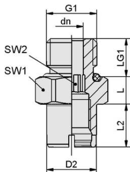
Design data SC-A 055 G1/4-AG L
