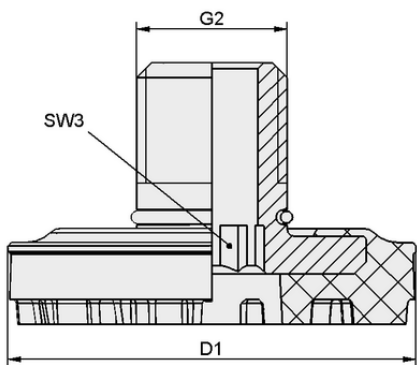
Design data SC-S 065 FDC-L
