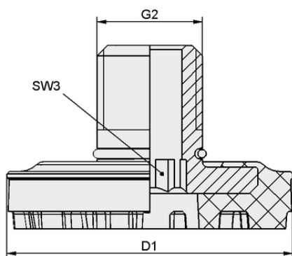
Design data SC-S 045 FDC-L
