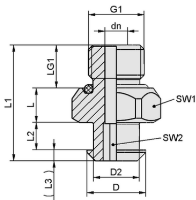
Design data SC 030 M5-AG
