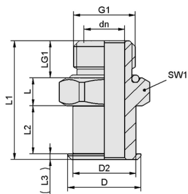
Design data SC 090 G3/8-AG
