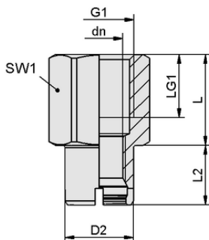
Design data SC-A 055 G3/8-IG L
