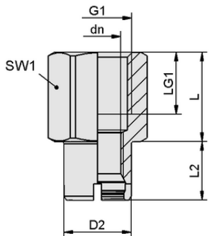
Design data SC-A 055 G1/4-IG L
