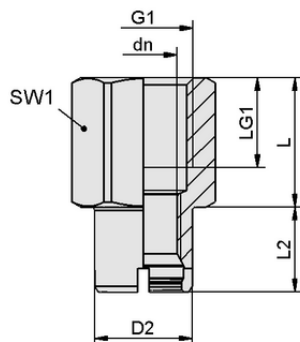
Design data SC-A 045 G3/8-IG L
