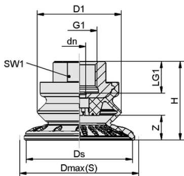
Design data SAB 80 HT1-60 G3/8-IG
