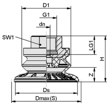
Design data SAB 40 HT1-60 G1/4-IG
