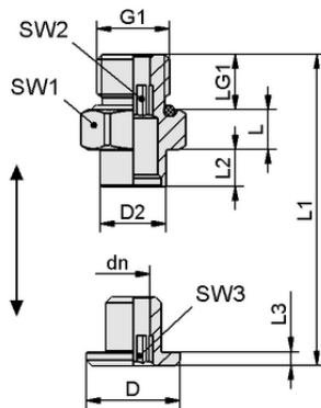
Design data SC 040-AR NPT1/8-AG MOD
