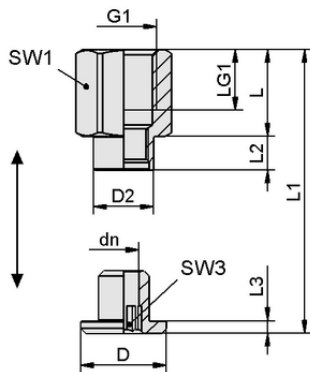
Design data SC 050-AR NPT1/4-IG MOD
