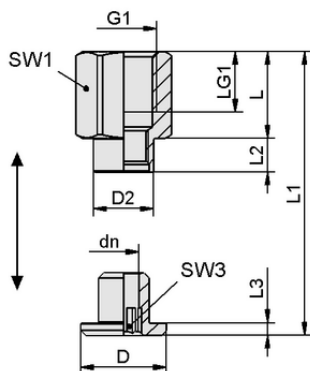
Design data SC 040-AR G1/8-IG MOD
