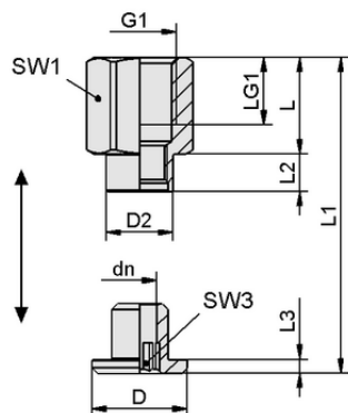
Design data SC 050-AR G1/4-IG MOD
