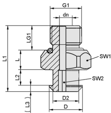
Design data SC 040 G1/8-AG
