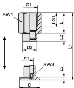
Design data SC 050 G1/4-IG MOD
