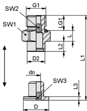
Design data SC 050 G1/4-AG MOD
