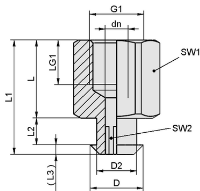
Design data SC 040 G1/8-IG
